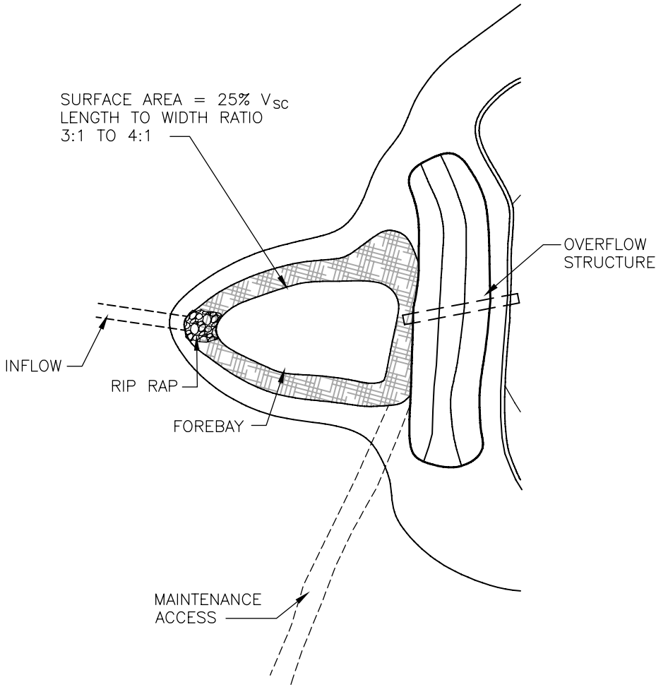
PLAN VIEW
