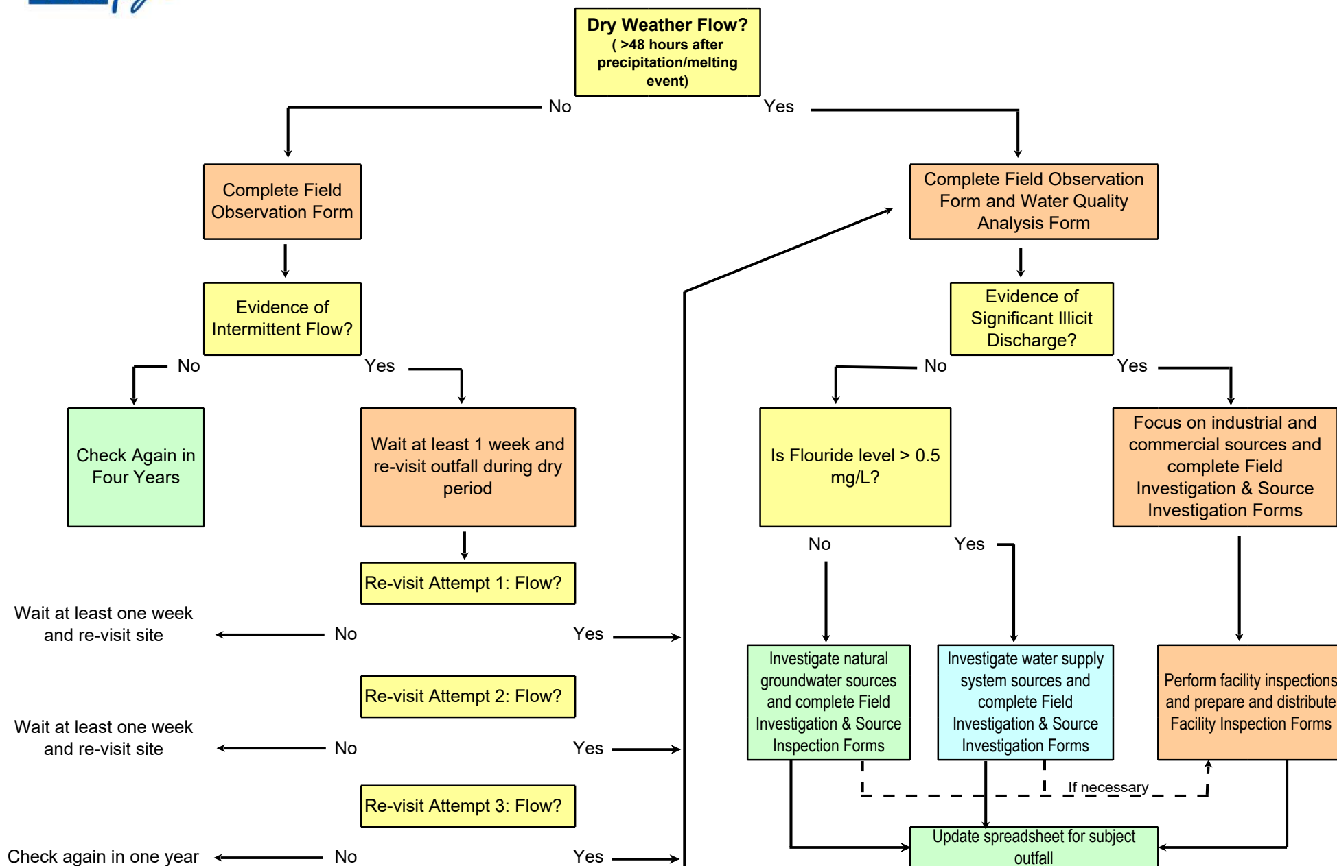
FIGURE 4 ACTION CHART FOR OUTFALL FIELD EVALUATION
